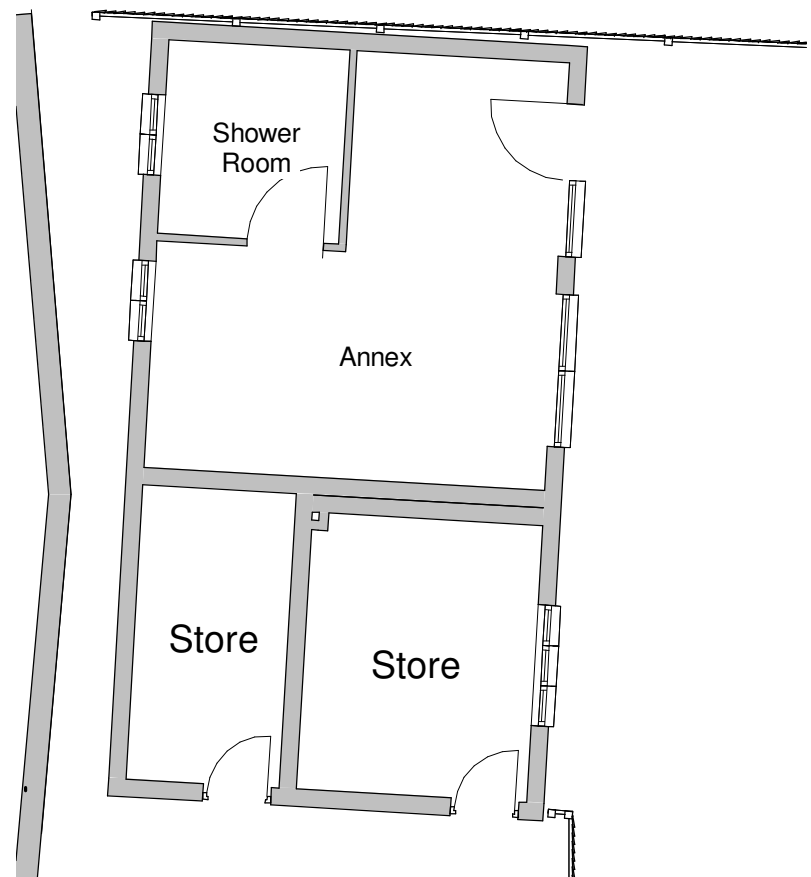
5 Garage Ground Floor 1 : 100
