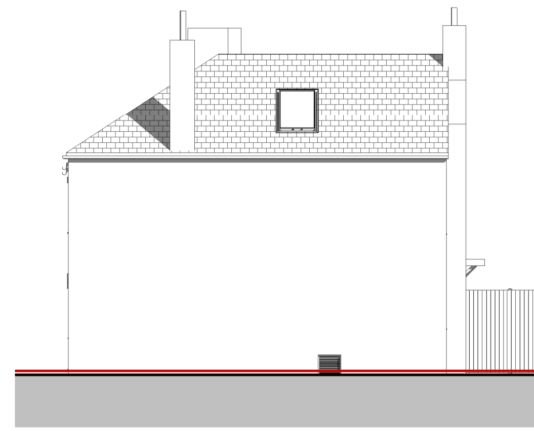
5 North Elevation 1 : 100
