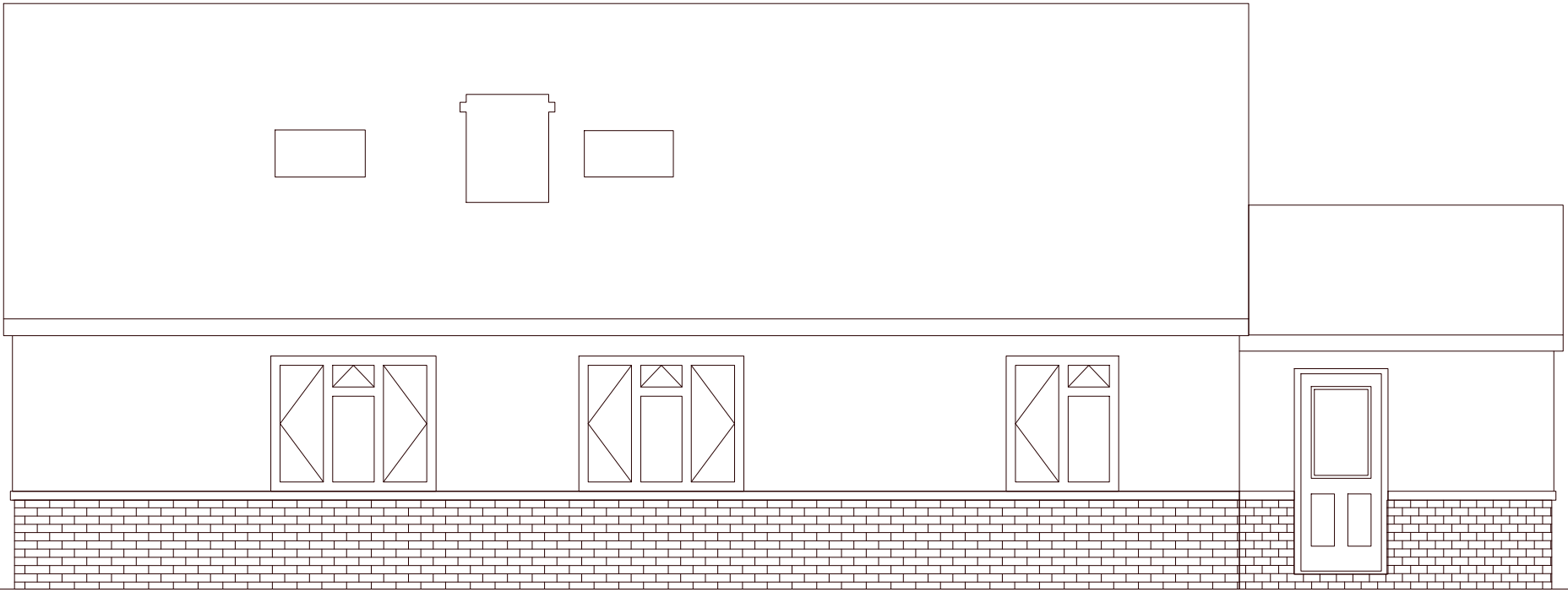
Right Elevation (Proposed) Scale 1:100 Printed at A4 Size
