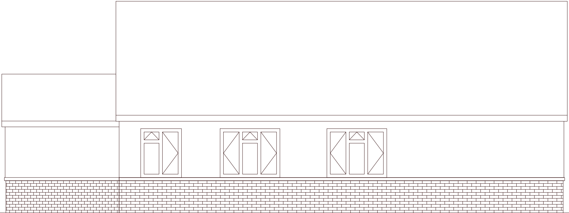
Left Elevation (Proposed) Scale 1:100 Printed at A4 Size
