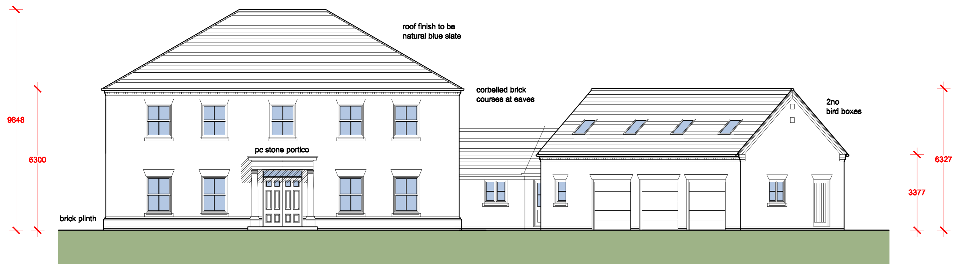
FRONT ELEVATION
