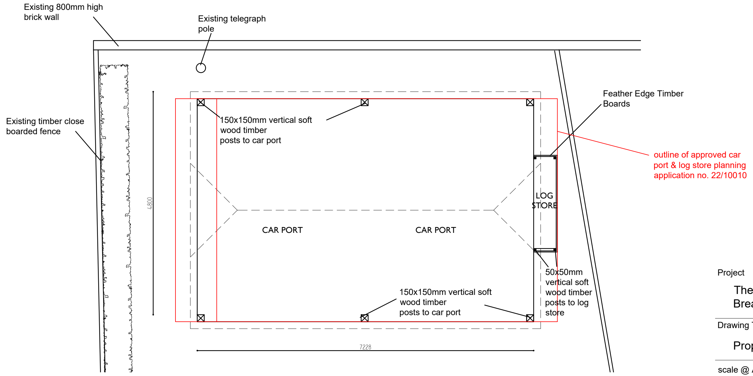
Plan scale 1:50
