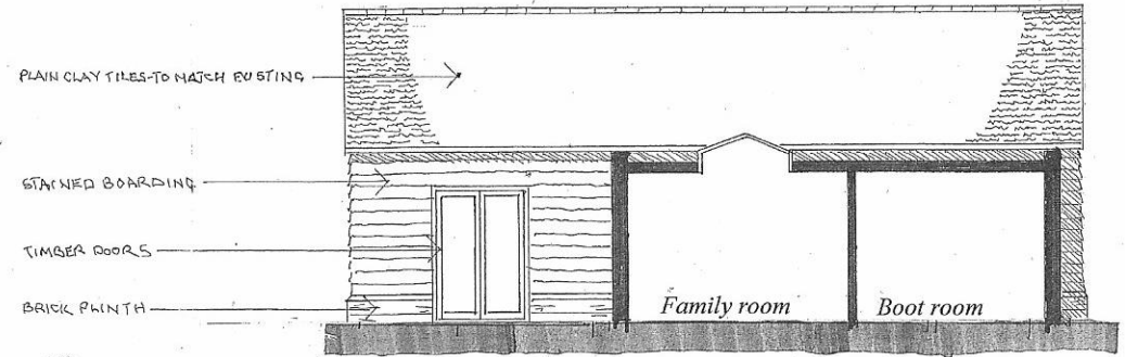
South West Elevation/Section
