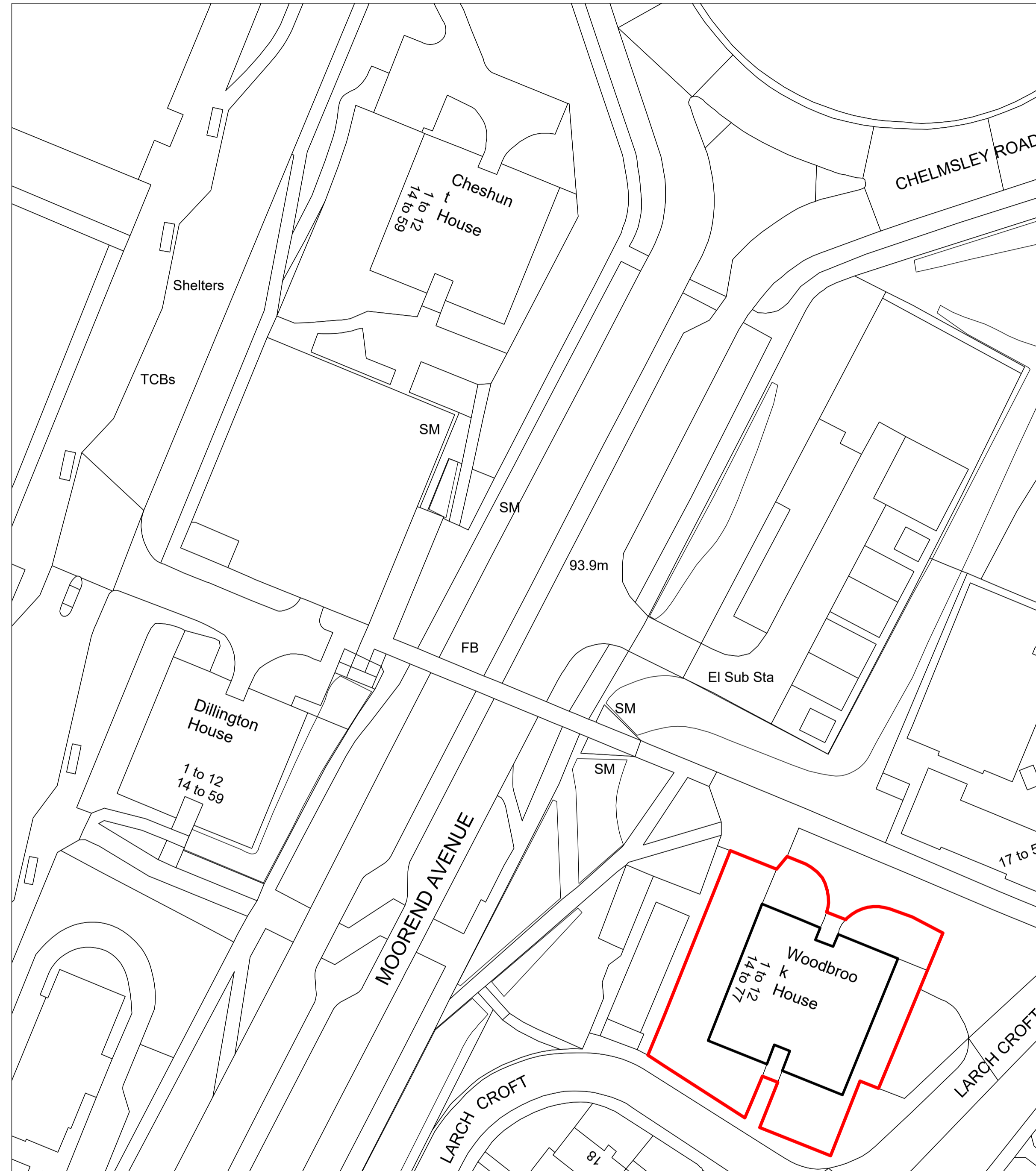
BLOCK PLAN
