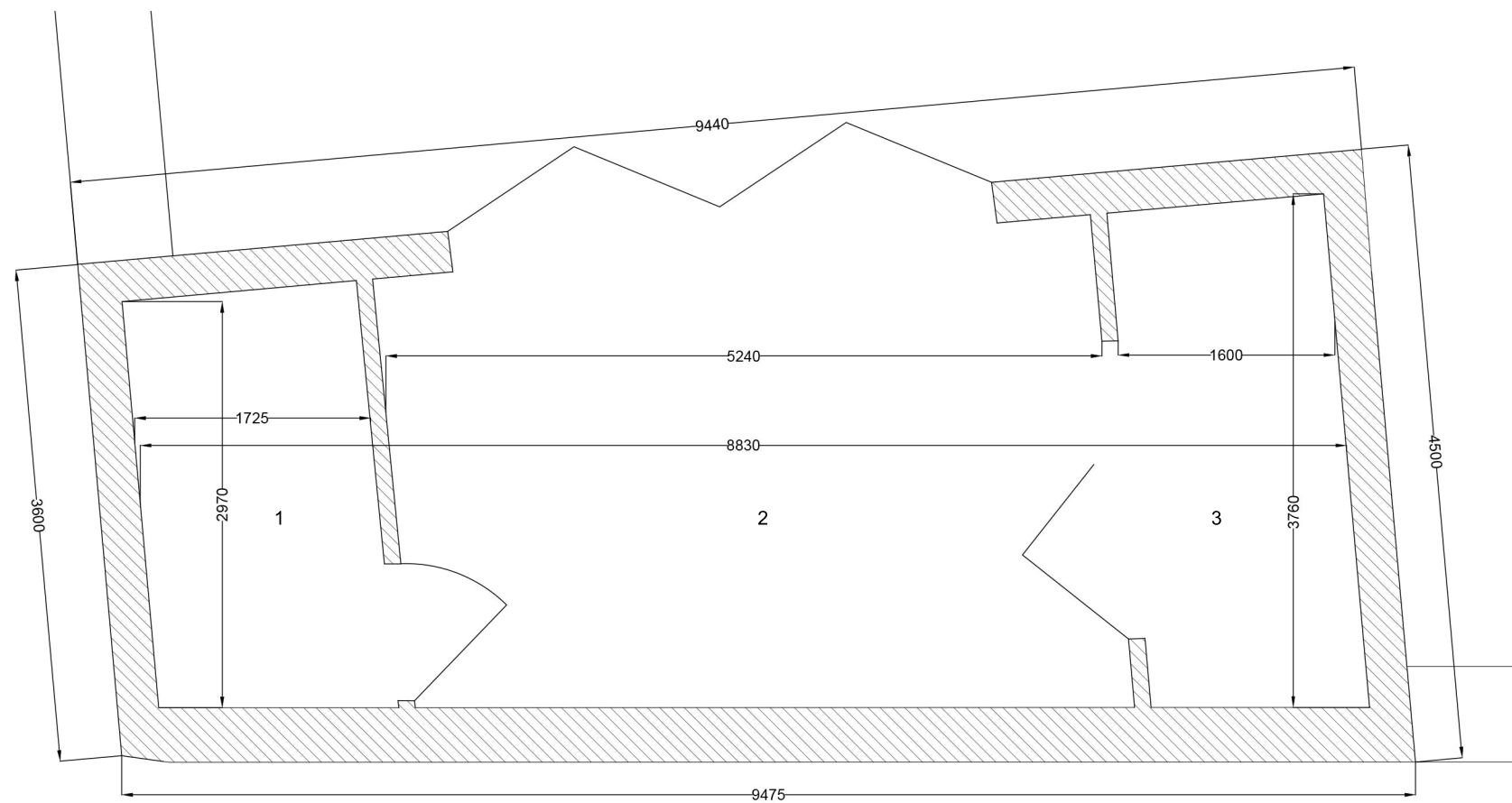
Floor Plan 1:50
