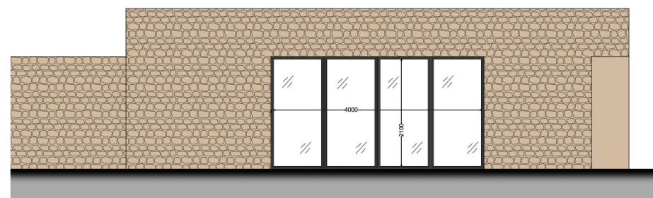
North Elevation 1:100
