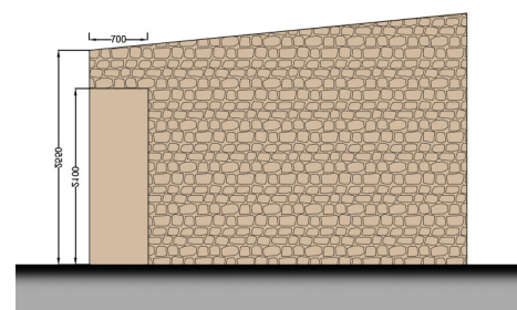
East Elevation 1:100
