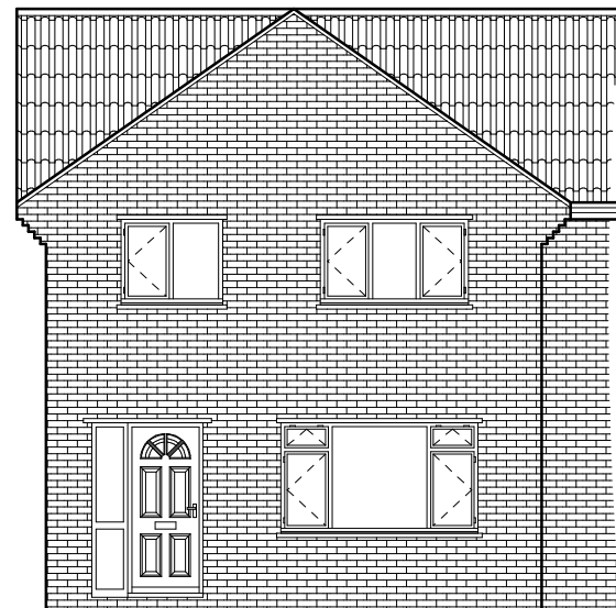
Front Elevation as Existing.
