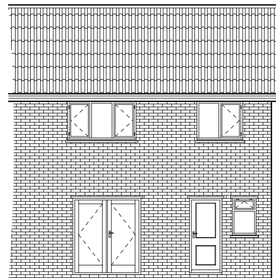
Rear Elevation as Existing.
