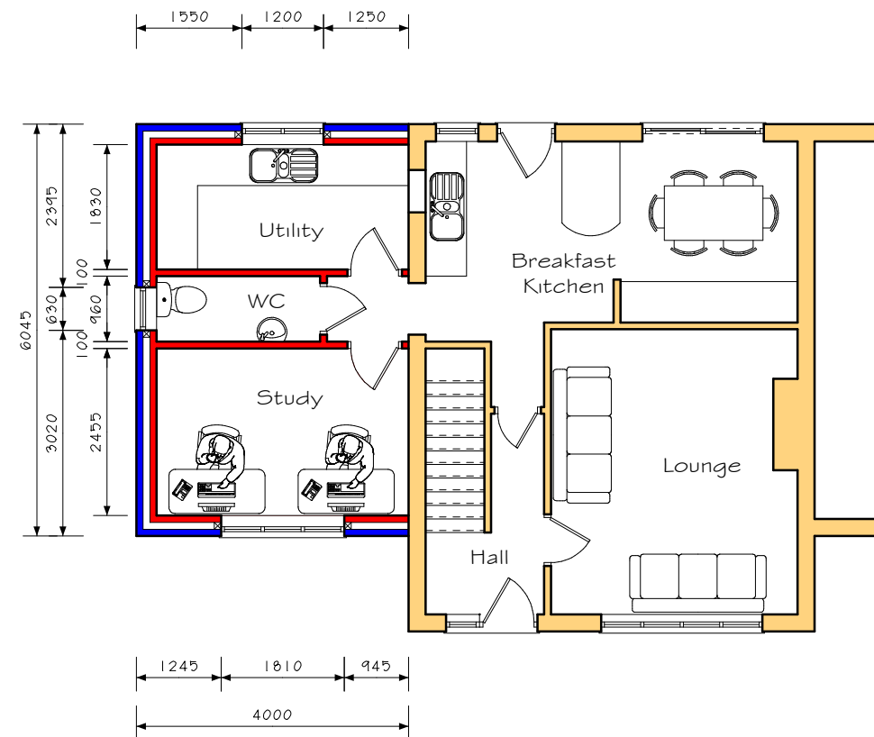
Ground Floor as Proposed.
