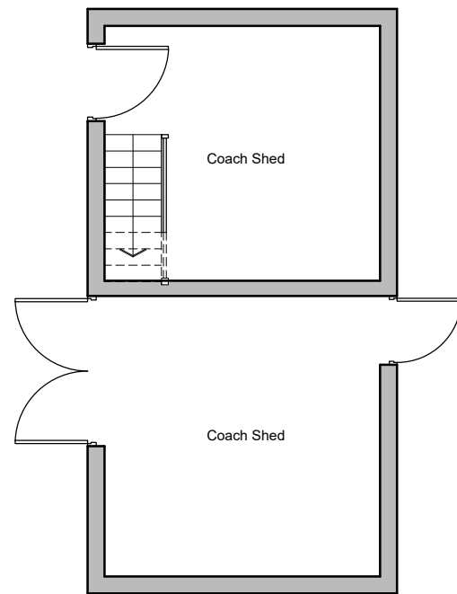
Existing Coach Shed Ground Floor
