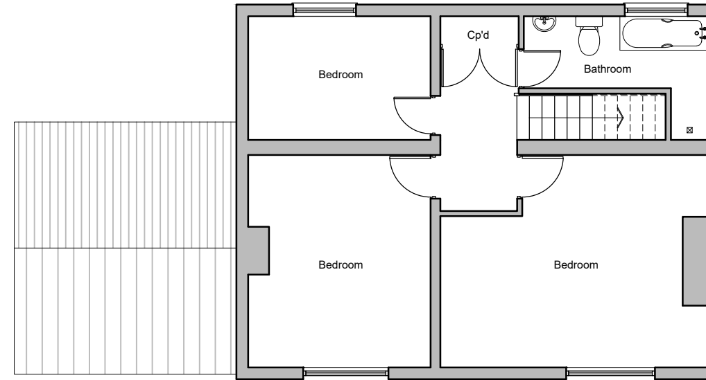
Existing First Floor Floor
