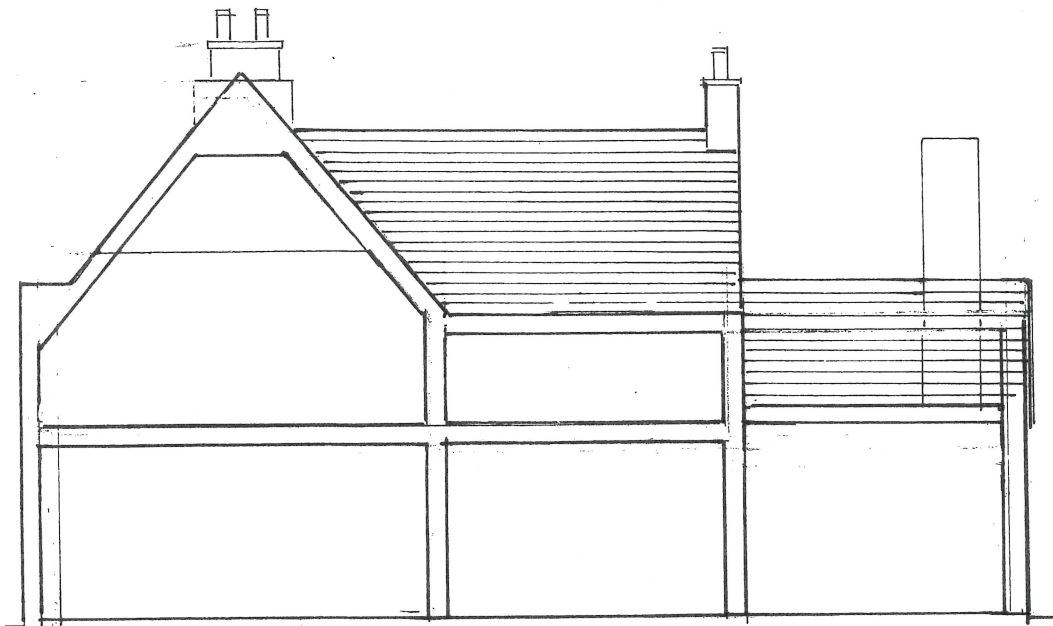
West Elevation as Existing
