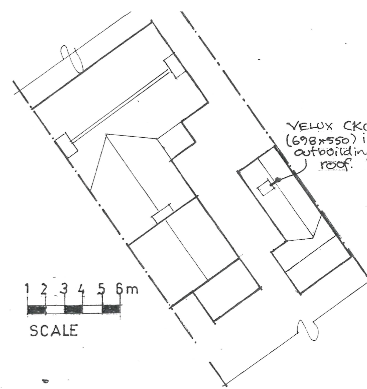
Roof Plan
