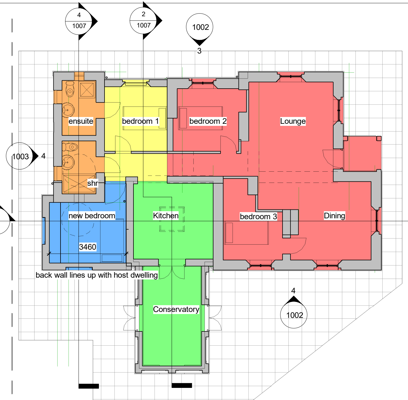
2 10 Ground Floor Plan Proposed 1 : 100
