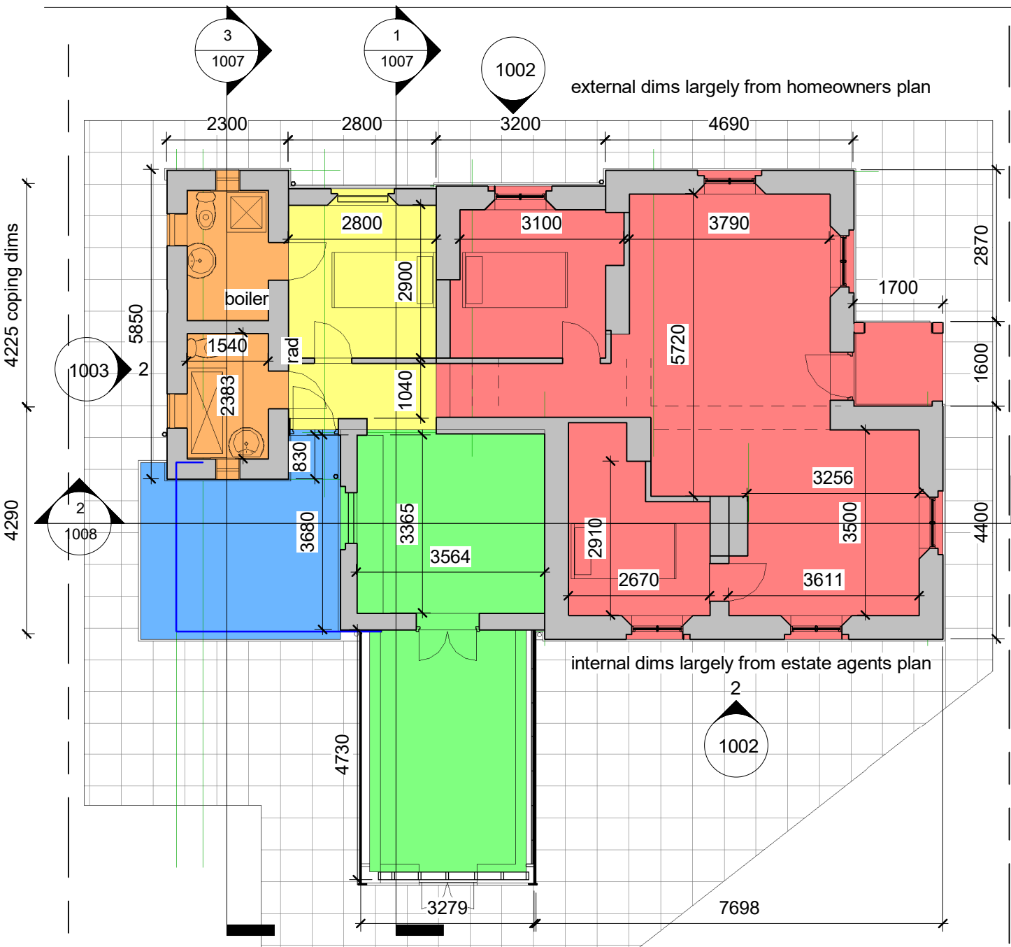
1 10 Ground Floor Plan Existing 1 : 100
