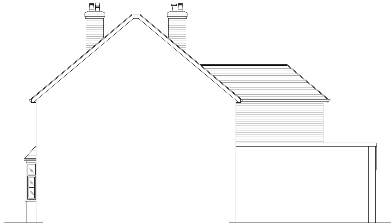
Right Side Elevation As Proposed
