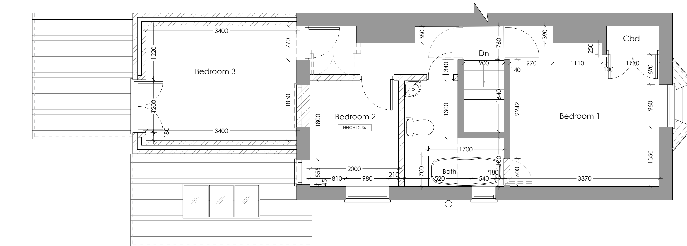
First Floor Plan As Proposed
