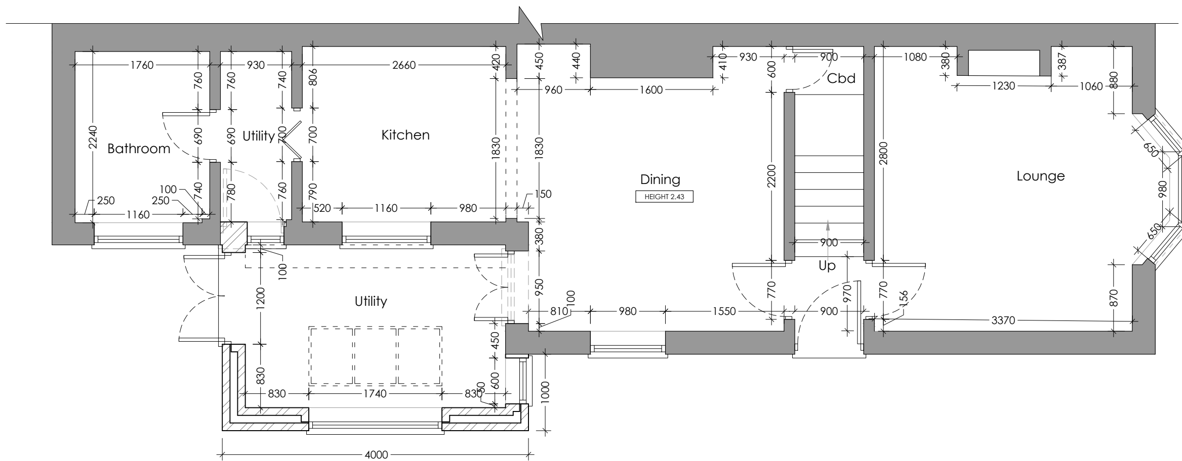
Ground Floor Plan As Proposed
