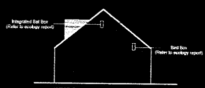
WEST ELEVATION
