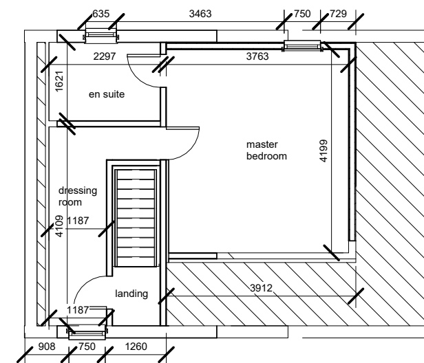
PROPOSED LOFT 1:100
