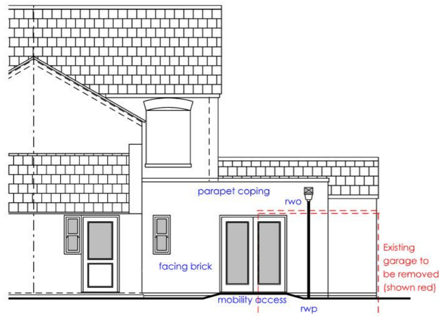
REAR ELEVATION (NORTH)
