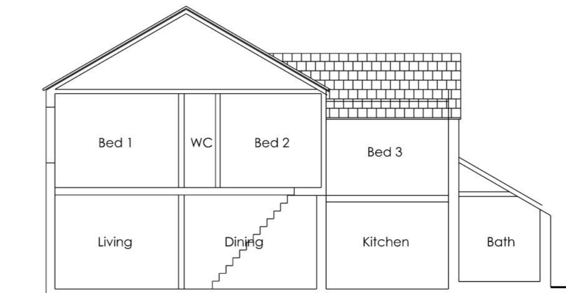
SECTIONAL SIDE ELEVATION (LOOKING WEST)
