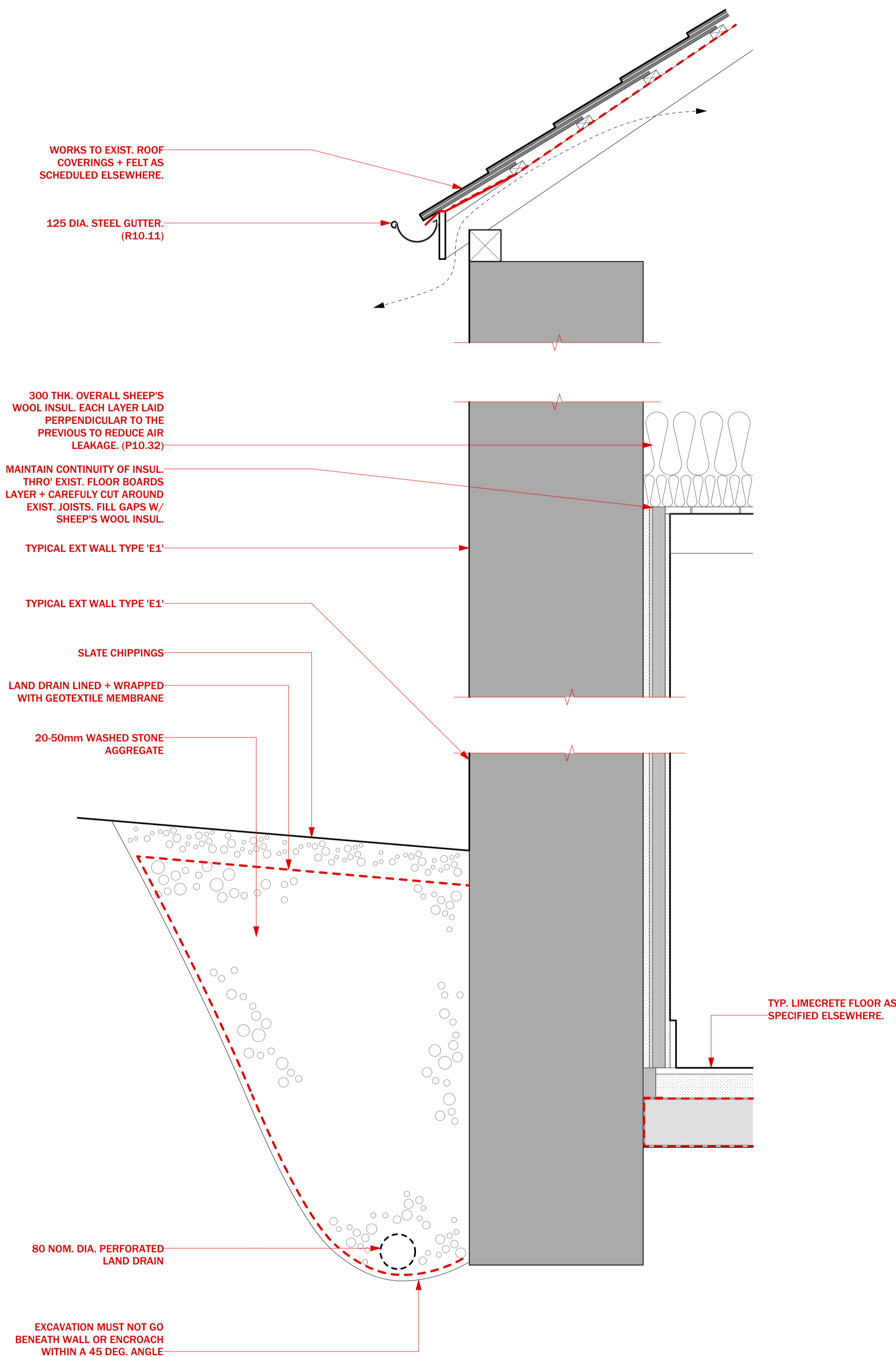
1 TYP. EXT. WALL @ STAFF BED '201' (NORTH) 1:10
