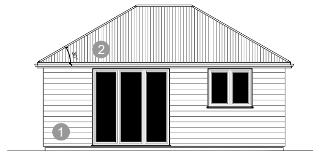
02 AS PROPOSED SIDE ELEVATION 1:100 @ A3
