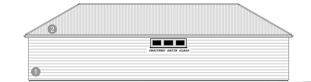
03 AS PROPOSED REAR ELEVATION 1:100 @ A3
