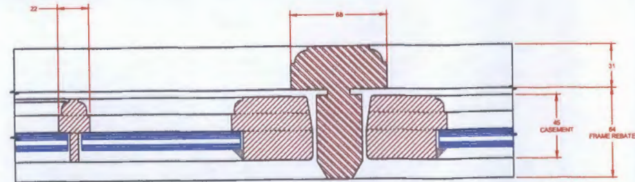
MULLION DETAIL
