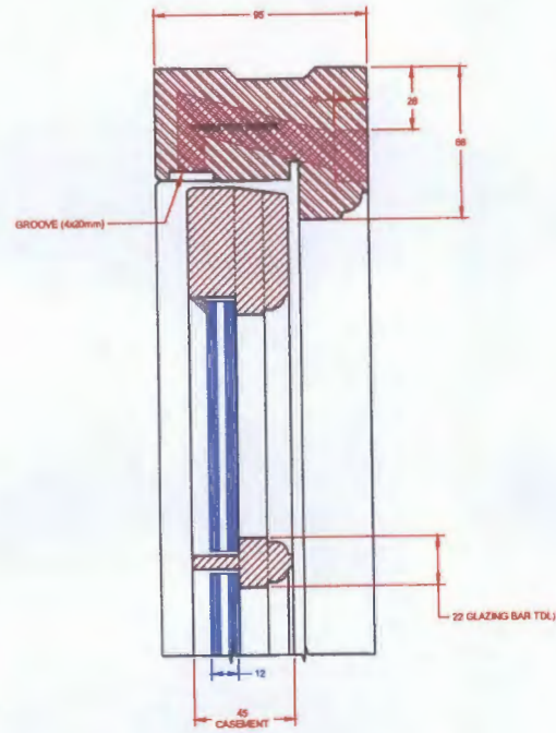
HEAD DETAIL
