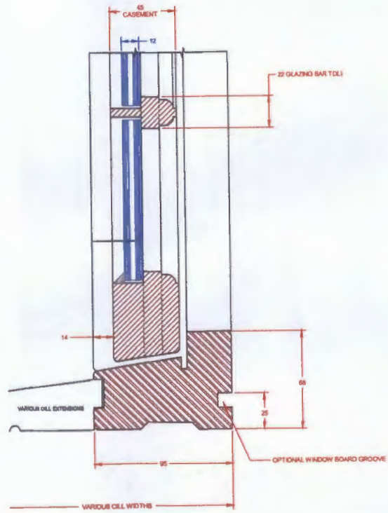
CILL DETAIL
