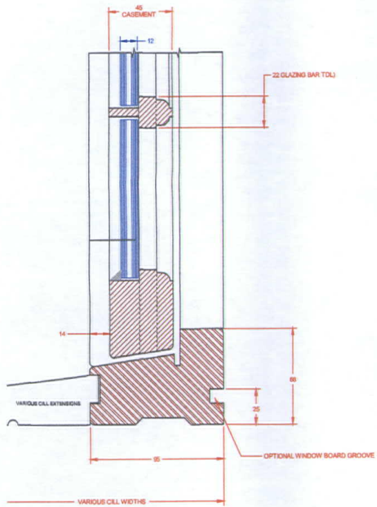
CILL DETAIL
