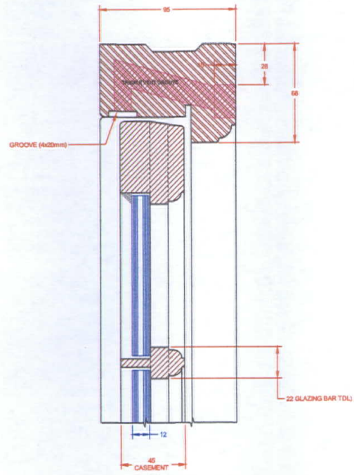
HEAD DETAIL
