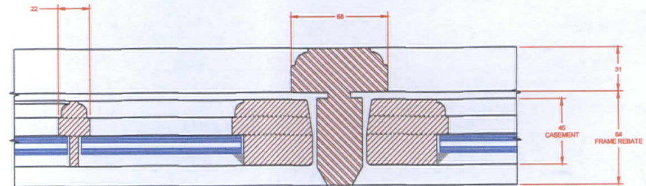
MULLION DETAIL
