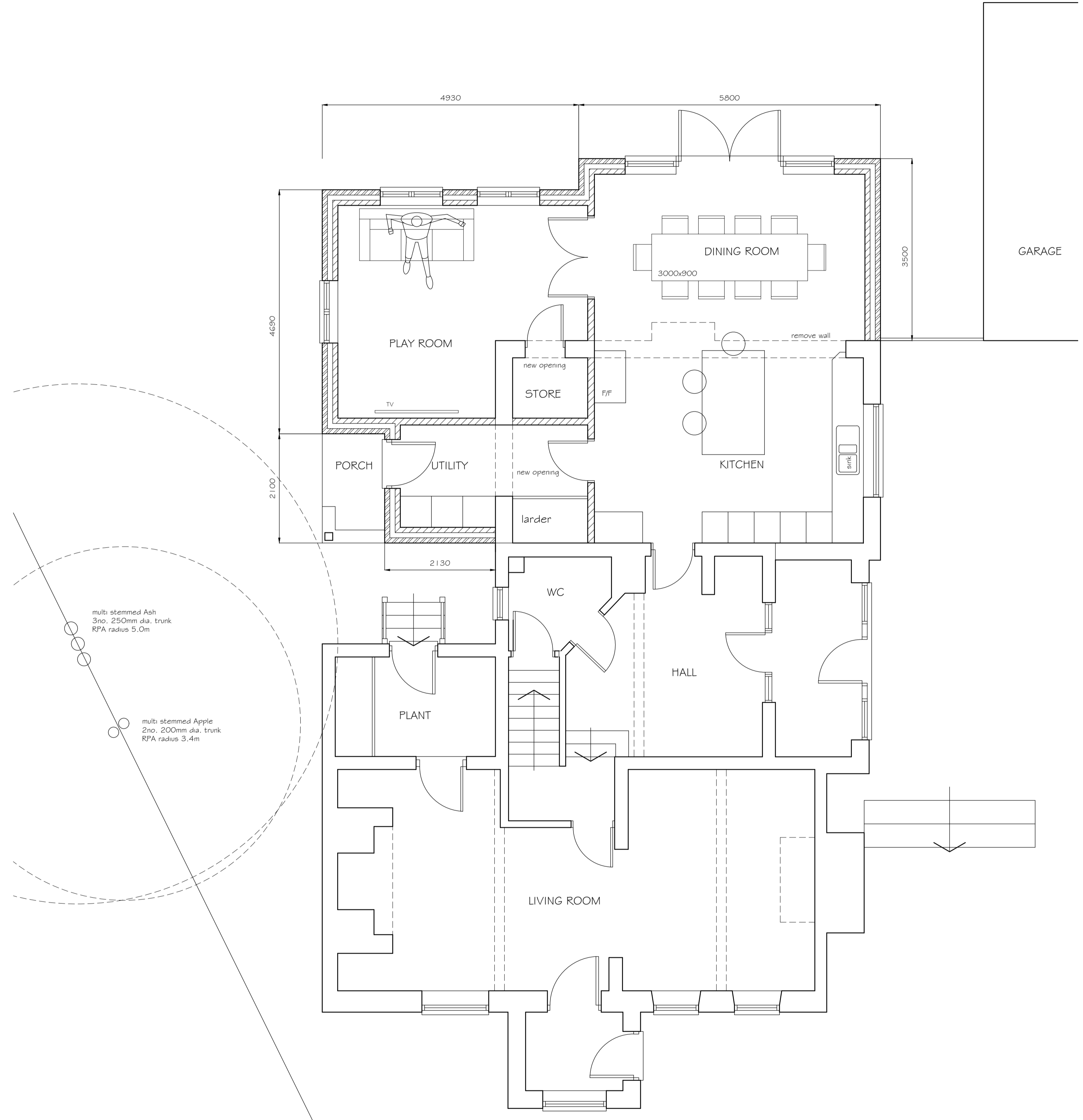
PROPOSED GROUND FLOOR SCALE 1:50 @A1 0 1 2 3 4m
