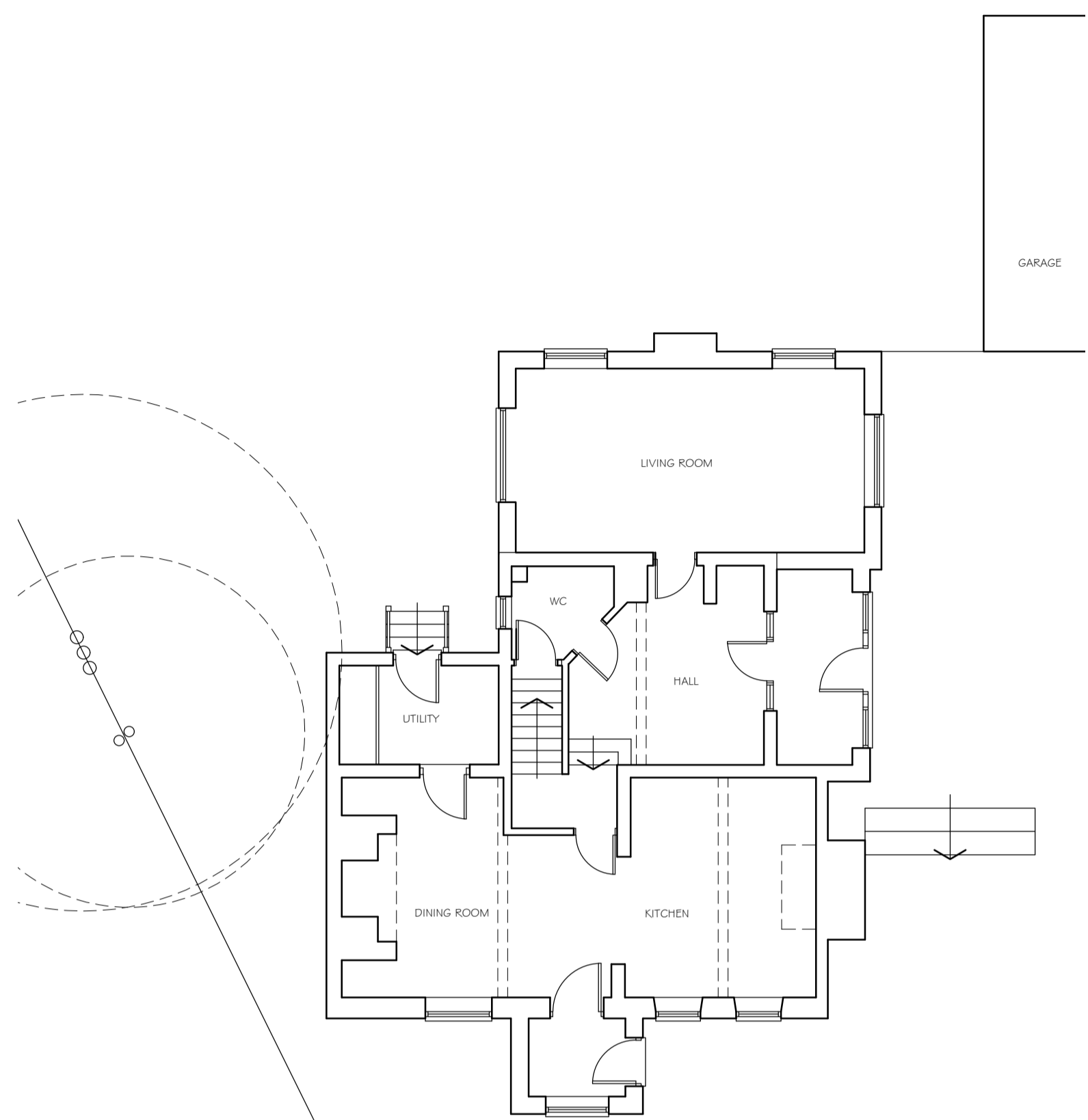
EXISTING GROUND FLOOR SCALE 1:100 @A1 0 1 2 3 4m
