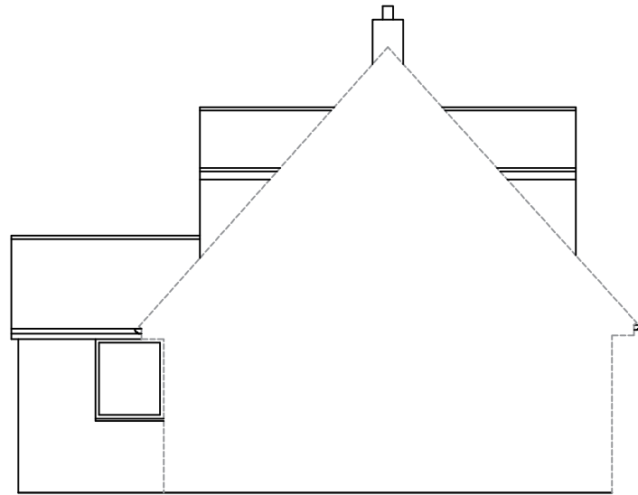
EAST ELEVATION
