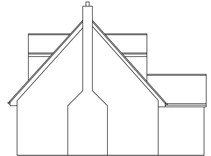
WEST ELEVATION
