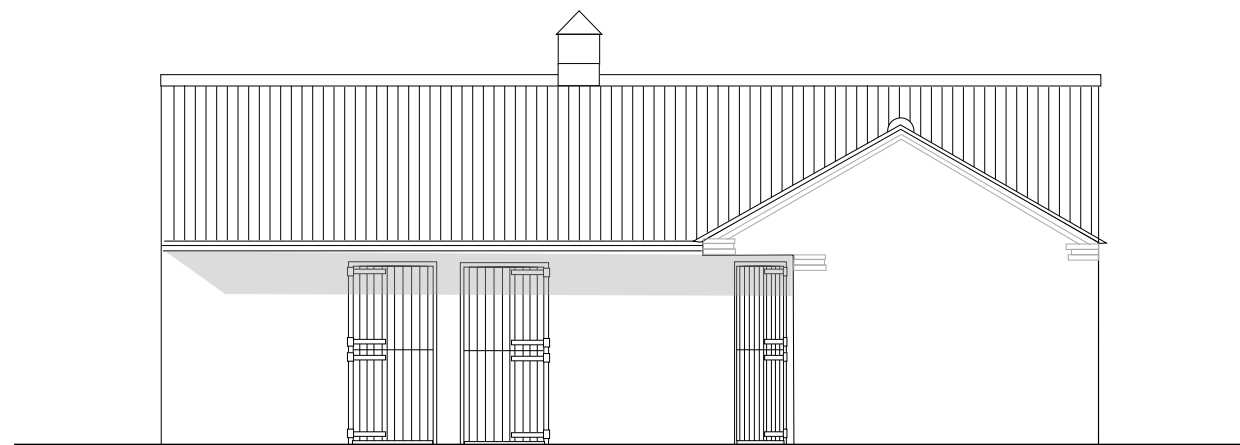
EAST ELEVATION 1:100
