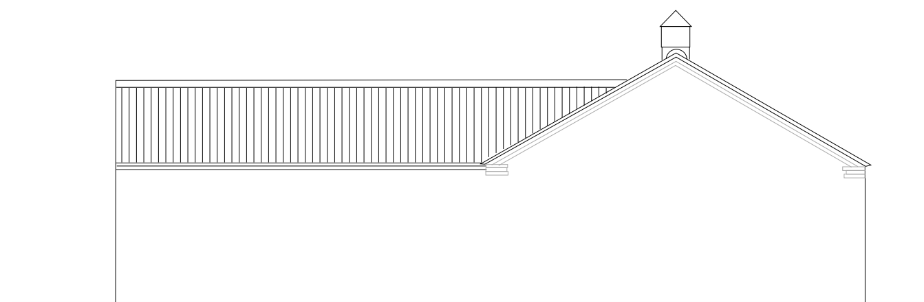
NORTH ELEVATION 1:100
