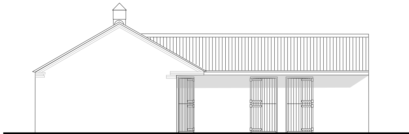
SOUTH ELEVATION 1:100
