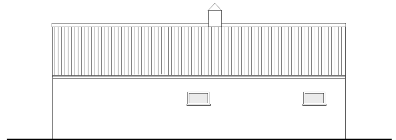
WEST ELEVATION 1:100
