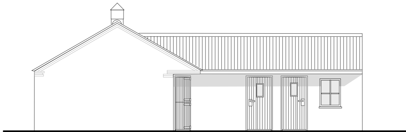
SOUTH ELEVATION 1:100
