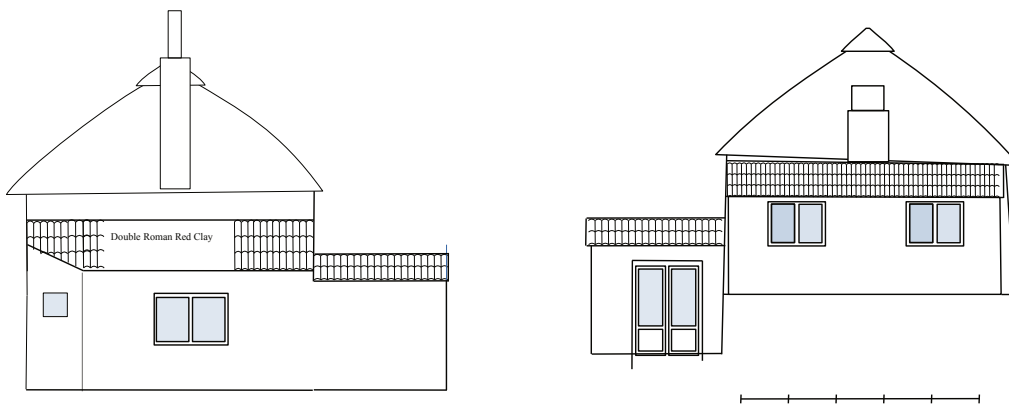
Honeysuckle Thatch, Talaton, EX5 2RN Proposed East and West Elevations Scale 1:100 Porch removed for clarity
