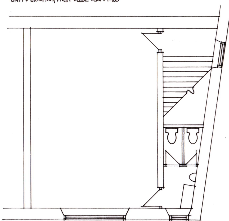
UNIT F EXISTING FIRST FLOOR PLAN 1:100
