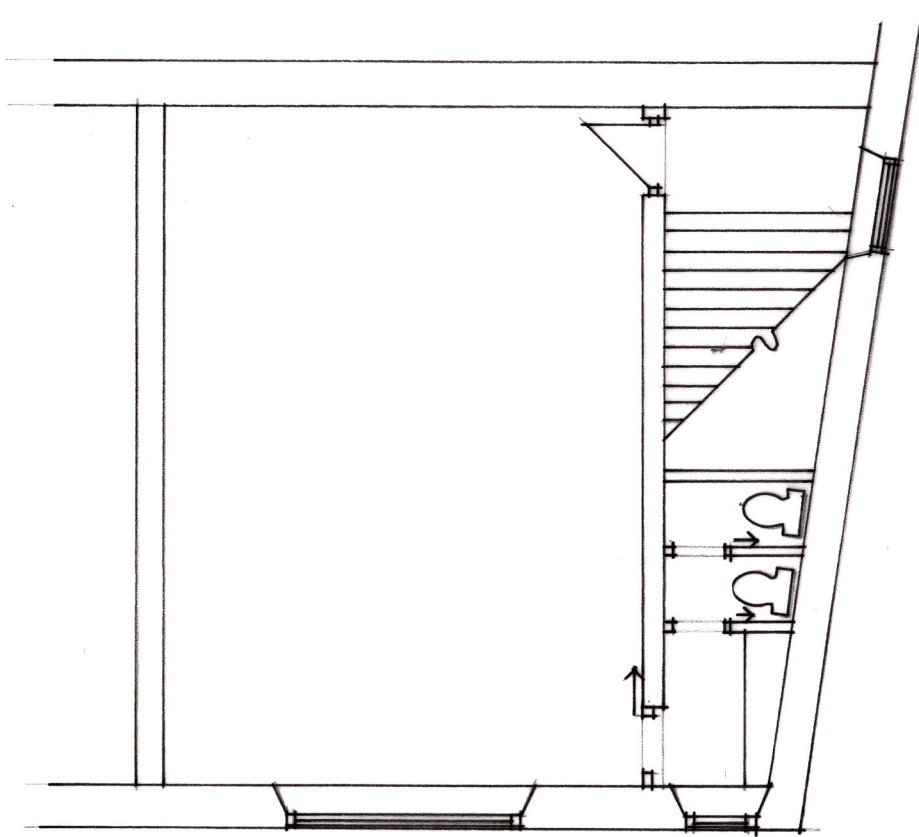
UNIT F EXISTING FIRST FLOOR PLAN 1:100
