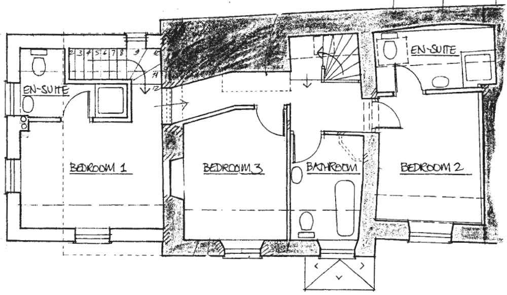
FIRST FLOOR PLAN 1:50
