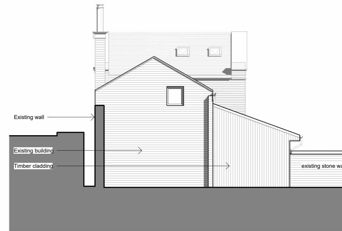
WEST ELEVATION 1:100
