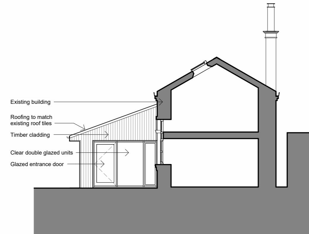
EAST ELEVATION 1:100
