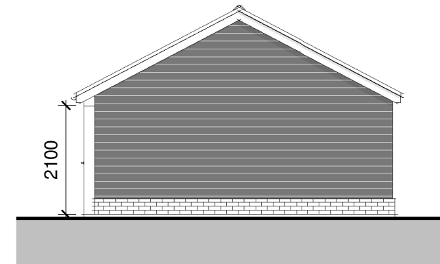
East Elevation As Proposed 1 : 100
