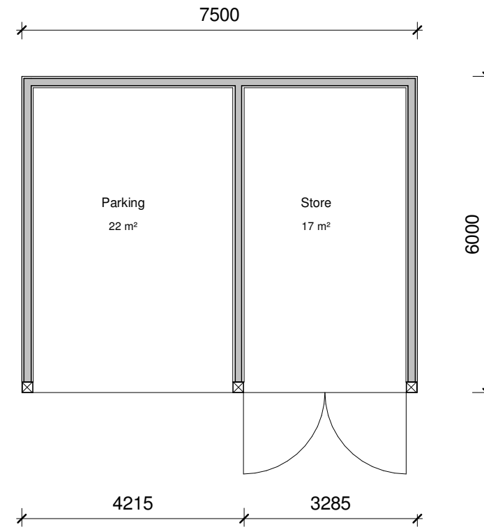
Ground Floor Plan As Proposed 1 : 100
