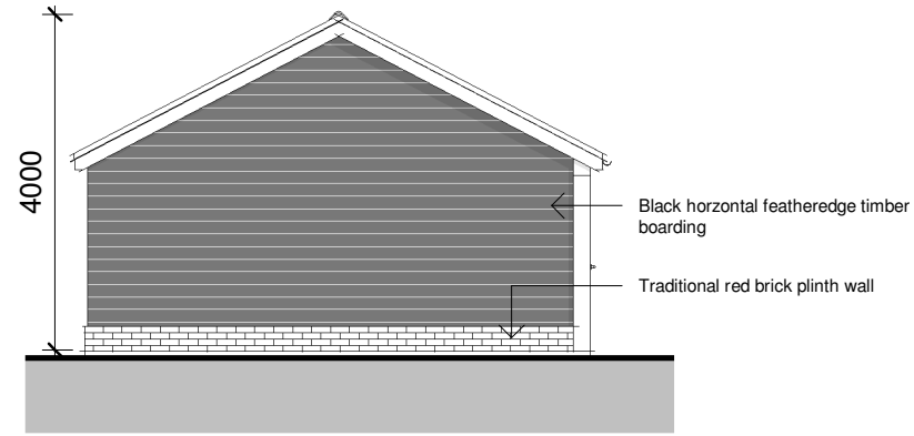
West Elevation As Proposed 1 : 100
