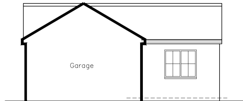
Side Elevation As Proposed (No change)
