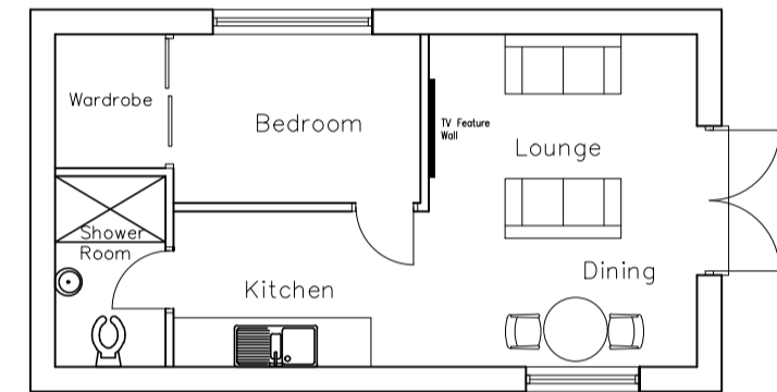
Ground Floor As Proposed
