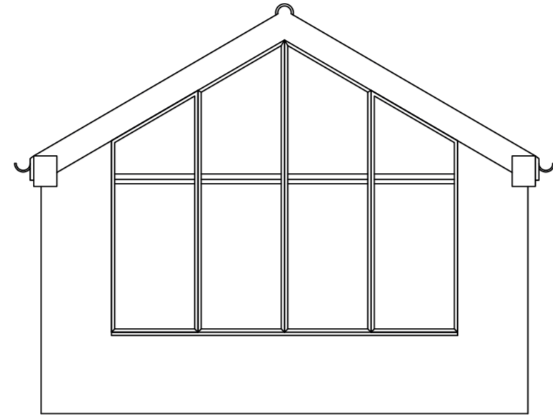
FRONT ELEVATION 1:50
