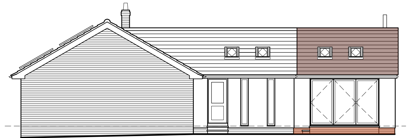
East elevation as existing
