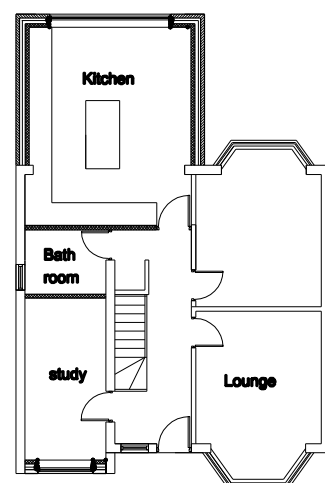
Proposed Ground Floor Plan
