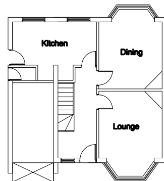
Existing Ground Floor Plan
