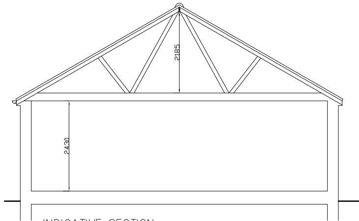
INDICATIVE SECTION
