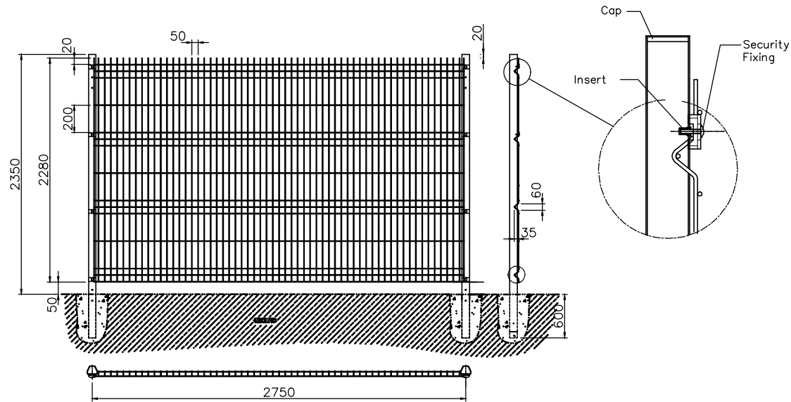
PROCTER FENCING SYSTEMS 2.4M HIGH PRO-MESH PANEL SYSTEM
