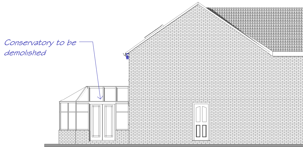
1 EXISTING Side (North West) Elevation 1 : 100
