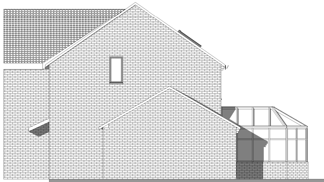
2 EXISTING Side (North East) Elevation 1 : 100
