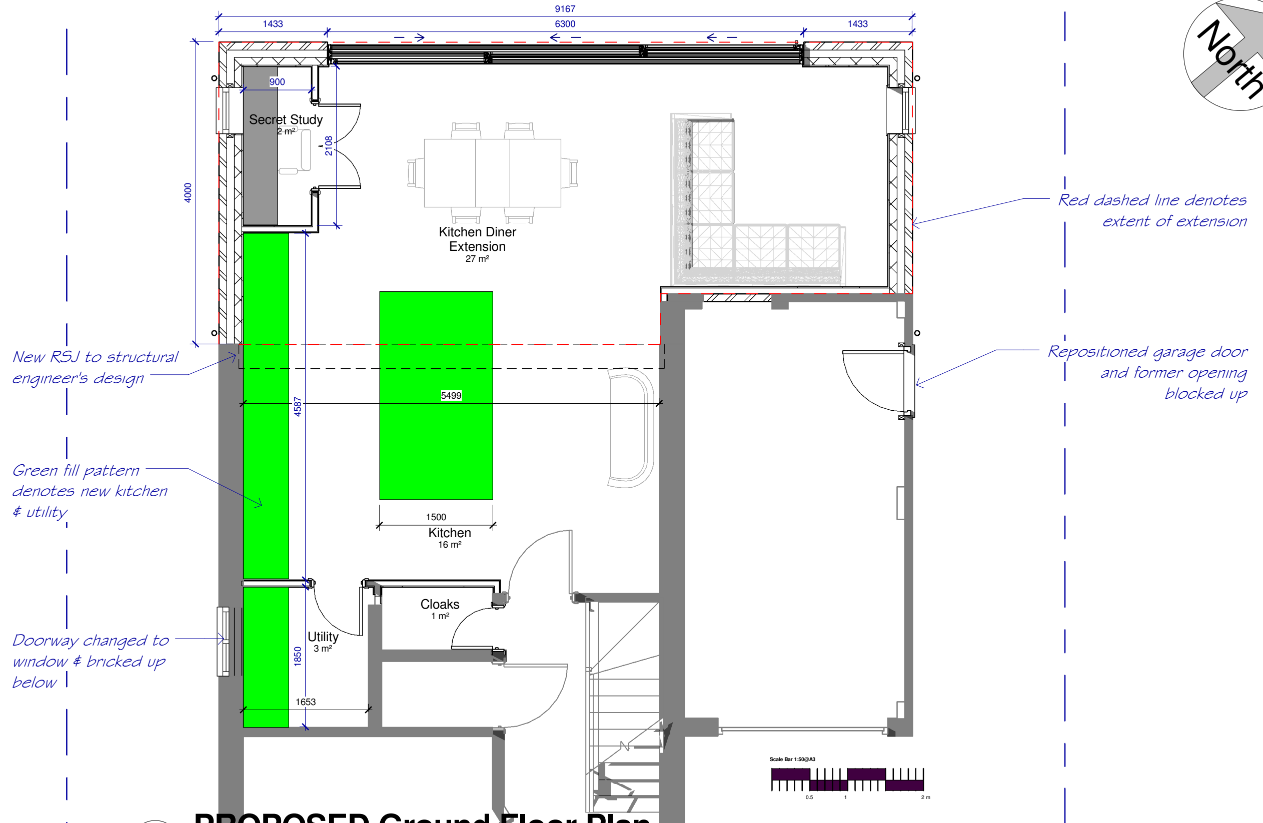
1 PROPOSED Ground Floor Plan 1 : 50
