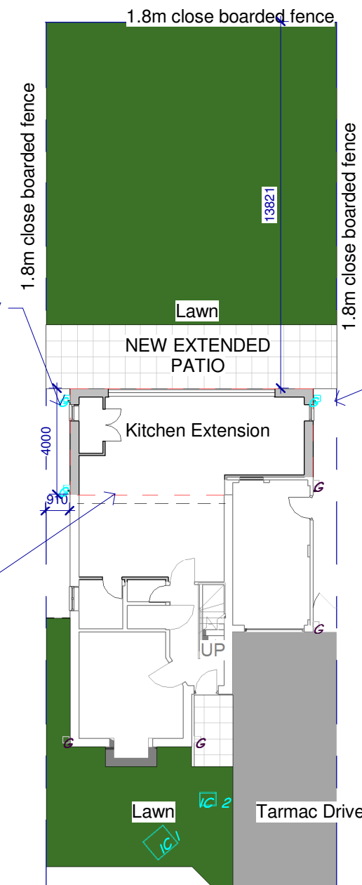
2 Proposed Site Layout 1 : 200
