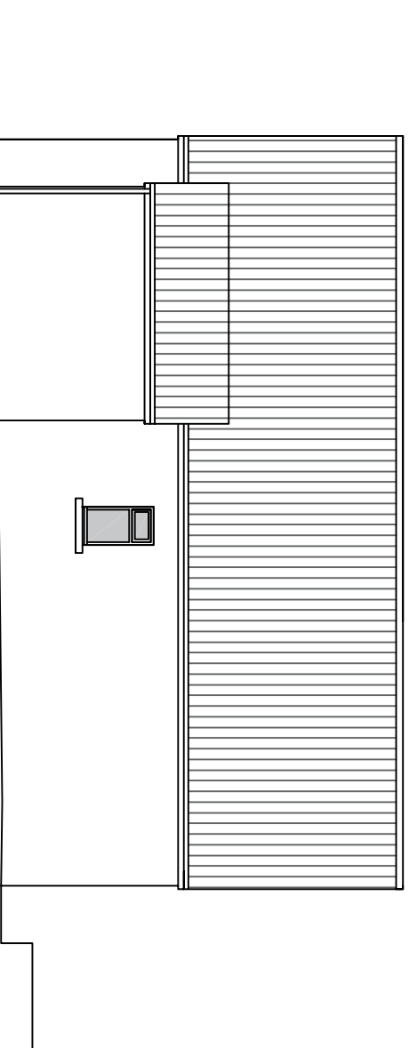
EXISTING NORTH-EAST ELEVATIONS 1:100
