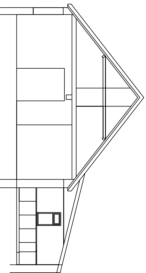
EXISTING TYPICAL SECTION 1:100
