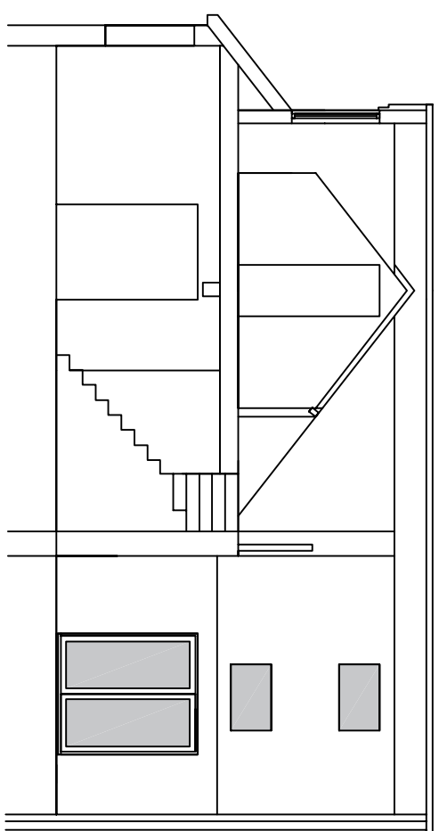
PROPOSED SECTION THROUGH LOFT CONVERSION 1:100
