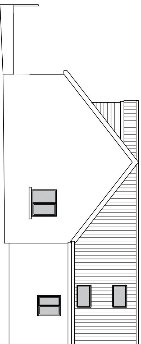
PROPOSED SOUTH-EAST ELEVATIONS 1:100
