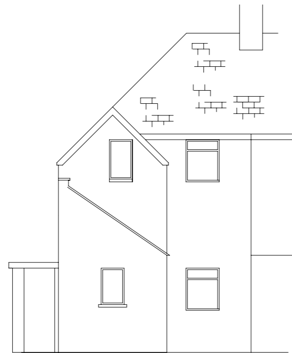
Existing Rear 1:100
