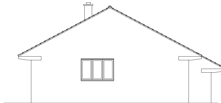
EXISTING WEST ELEVATION SCALE - 1:100 @ A3
