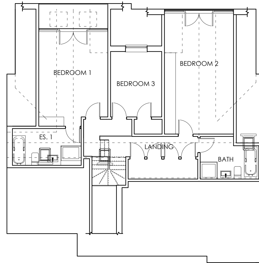
PROPOSED FIRST FLOOR PLAN SCALE - 1:100 @ A3
