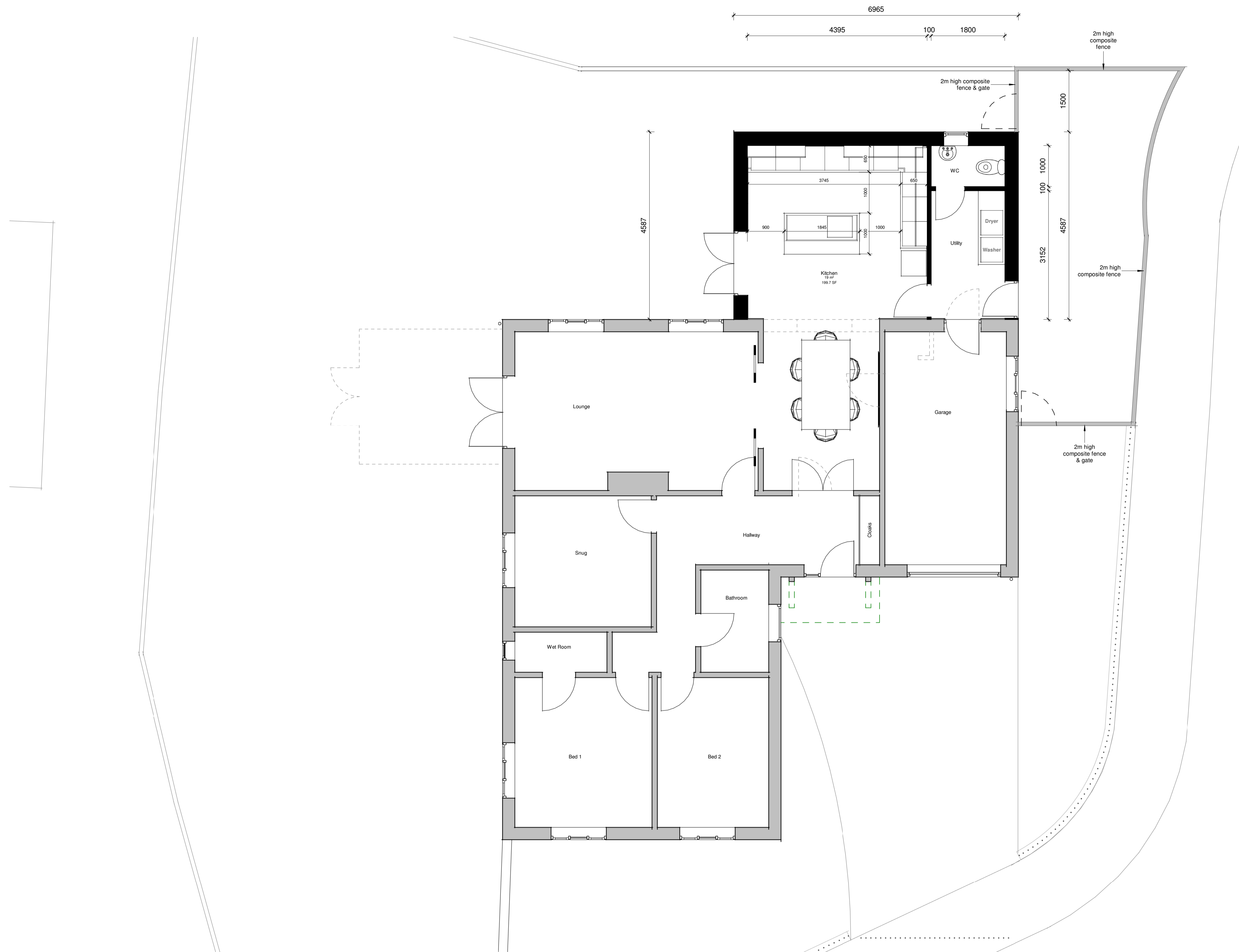
Ground Floor 1 : 50
