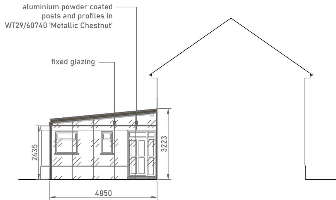
SIDE SECTION
